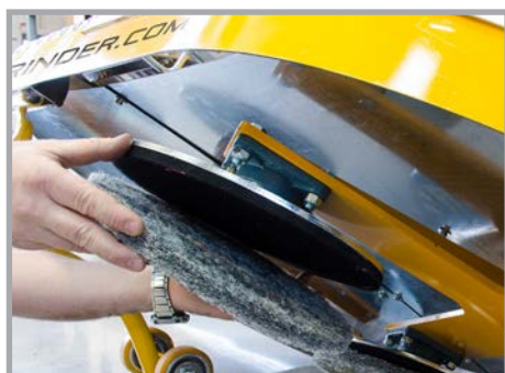
Tools holder with ø300 mm velcro attach
